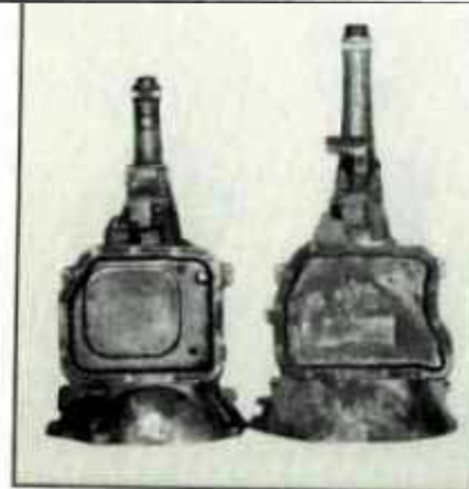
The A-727 transmission on the right is nearly 4 inches longer than the A-904 on the left. Also, note the difference in the shape of the pans. The A-727 has a hump on the passenger's side near the front.
